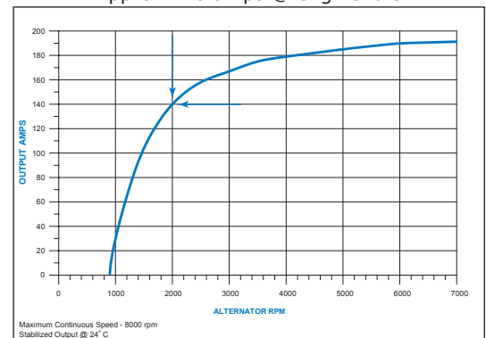
Graph B Leece-Neville 185 amp alternator Approx 140 amps @ engine idle
