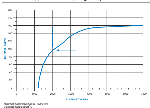
Graph A Leece-Neville 160 amp alternator Approx 95 amps @ engine idle
